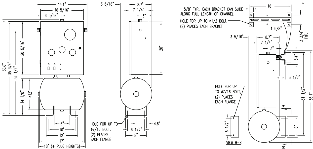
Figure 2 - Dimensions for the 655 Series BlendMaster™
