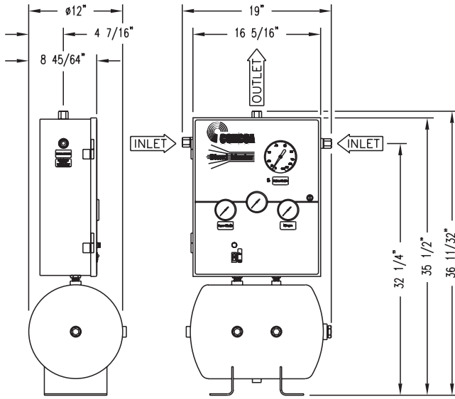
Model 1000 Floor-Mounted
