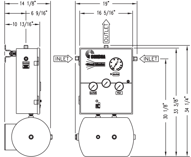
Model 1000 Wall-Mounted
