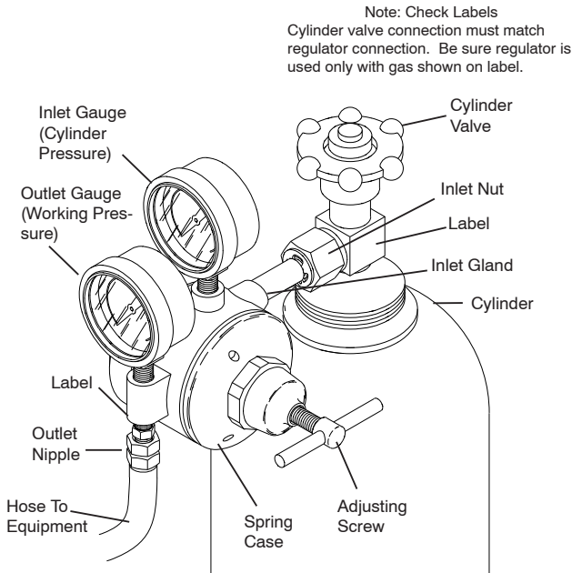
Figure 2. Typical Regulator and Connection to Cylinder
